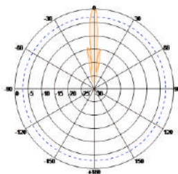
H-Pol Elevation
